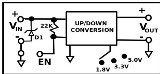
Figure 3 – Electrical Schematic for X0122 Converter
