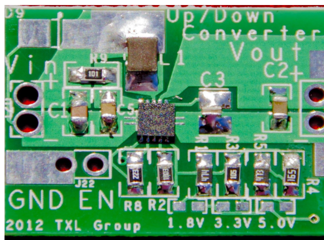
Figure 2 – The X0122 Up/Down Converter
